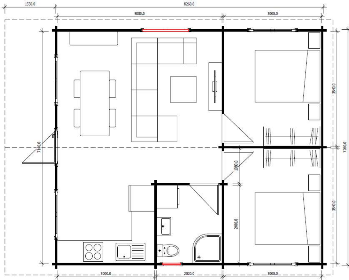
— — - customizable placement of windows marked red on the floor plan
